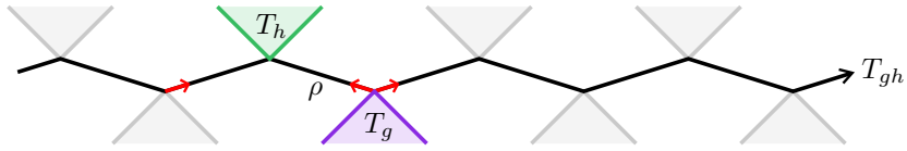
FIGURE 7. Case I, g and h elliptic. T_h is green, T_g is purple, T_{gh} is black. The red edges are of the form e , he , and ghe .
