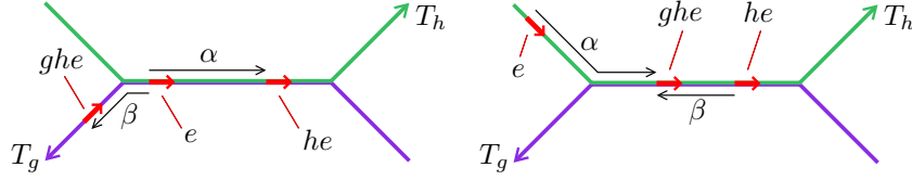
FIGURE 9. Cases III-C (left) and III-D (right). T_h is green, T_g is purple.
