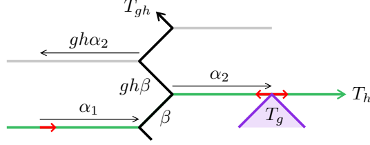
FIGURE 10. Case IV. The element gh takes \alpha_1 to \bar{\alpha}_2 . Left to right, the red edges are h^{-1}e , ge , and e .
