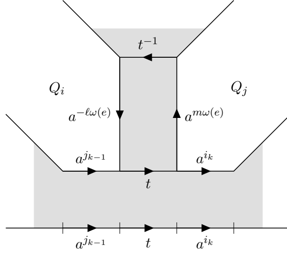
FIGURE 4. Using the polygons Q_i to build a band surface S_0 . The surface S_0 is shaded above.
