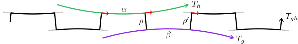
FIGURE 6. Case I, g and h hyperbolic. T_h is green, T_g is purple, T_{gh} is black. The red edges are of the form e , he , and ghe .
