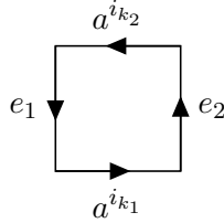
FIGURE 3. A sample polygon corresponding to a circuit \gamma of length 2.
