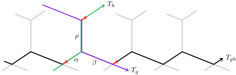
FIGURE 8. Case III-A. T_h is green, T_g is purple, T_{gh} is black. The red edges are of the form e , he , and ghe .
