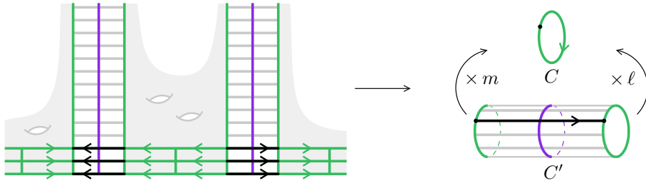
FIGURE 1. An admissible surface after the transversality procedure. The gray regions map into C .
